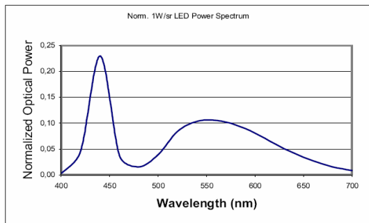
Fig. 4 Spectrum characteristic of White LED [1]
