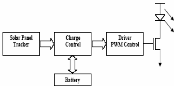
Fig. 6 System block diagram
