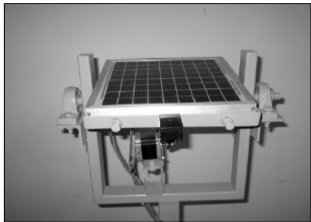
Fig. 10 Tracking system for solar module
