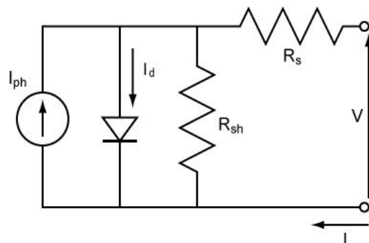
Fig. 1 Solar cell equivalent circuit
