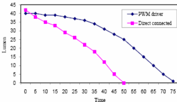
Fig. 9 Comparisons of Directed connected and PWM driver
