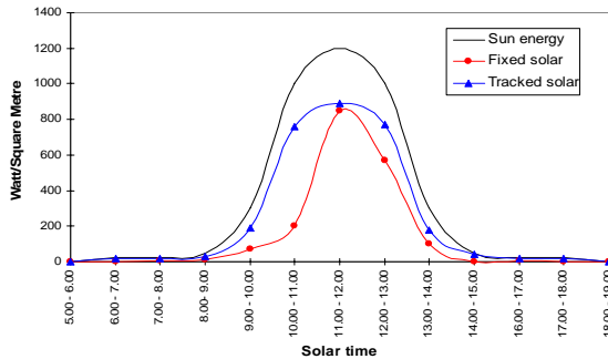
Fig. 8 Fixed and Tracking solar power energy
