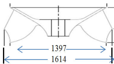
Fig. 17 (a) High Ns impeller [27]
