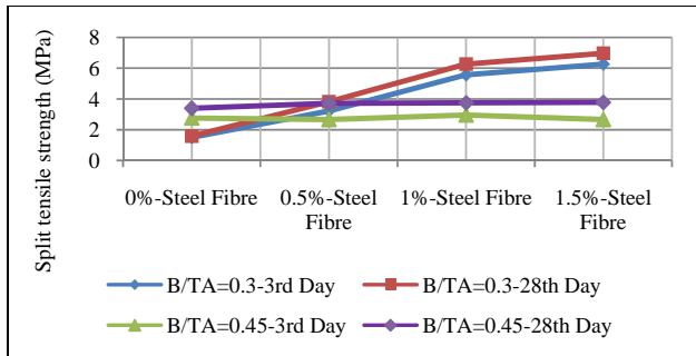
Fig. 3 Split tensile strength property of steel fibre reinforced geopolymer concrete
