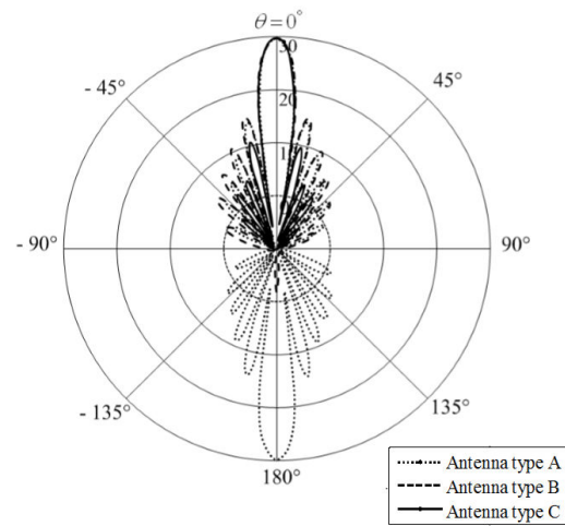
(a) E-Plane
