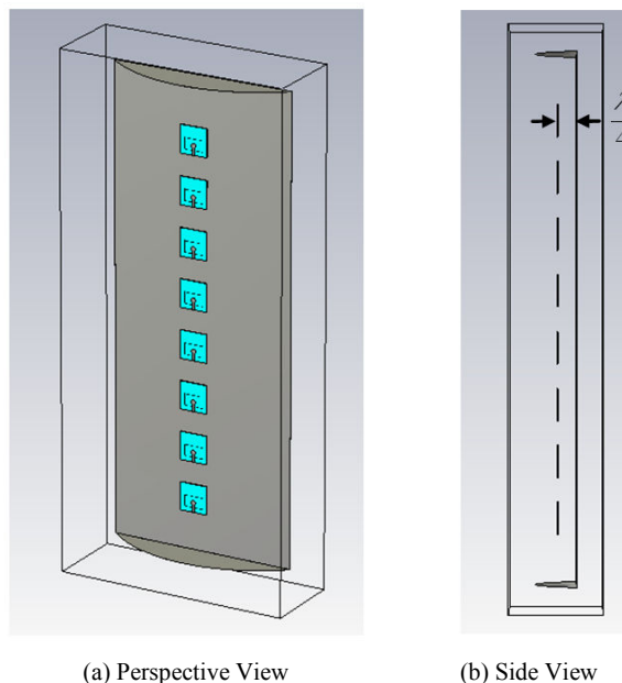
Fig. 2 A 1×8 array of circular MSAs and U-shaped reflector (antenna type B)
