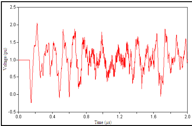
Fig. 2 VFTO at transformer terminals Tr1
