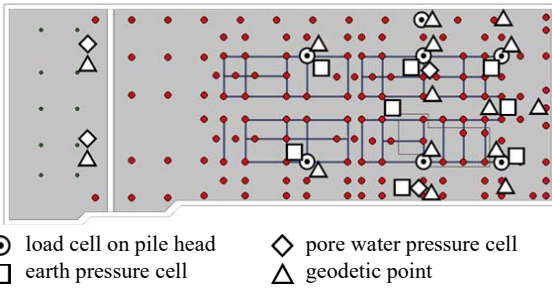
Fig. 6 Monitoring instrumentation
