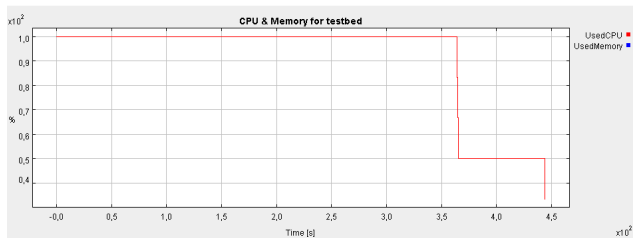
Fig. 10 Shortest job first Scheduler (50 tasks)
