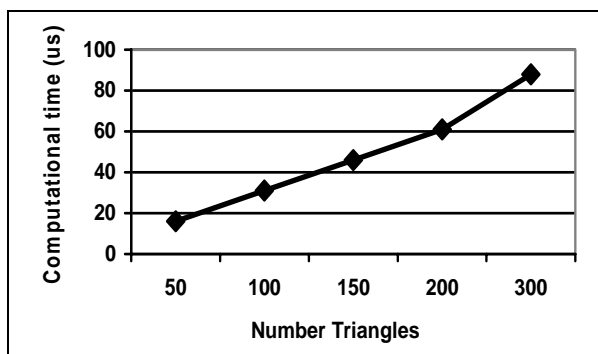
Fig. 6 Computational time for the “segment-triangle” procedure (no collision)
