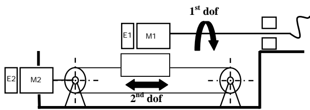
Fig. 8 Scheme of the HERMES haptic interface
