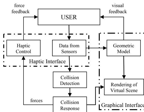
Fig. 2 Architecture for the HERMES simulator
