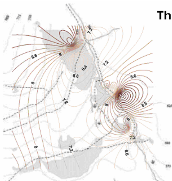
Fig. 2 Distribution of the Cu, As and Th contamination of the dump-field sediments at the Cubietová deposit. The number indexes on the isolines represent the concentration in ppm
