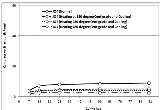
Fig. 7 The compressive strength of the concrete mix JO4 at normal condition and when subjected to heating
