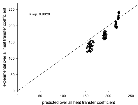
Fig. 7 Comparison of experimental data with present data of 10.41 cm pitches coil
