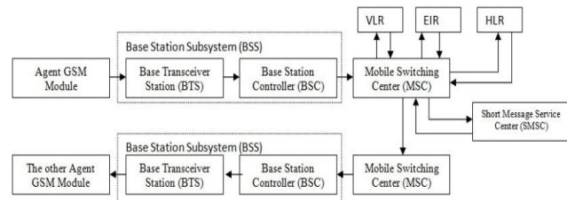
Fig. 5 SMS architecture
