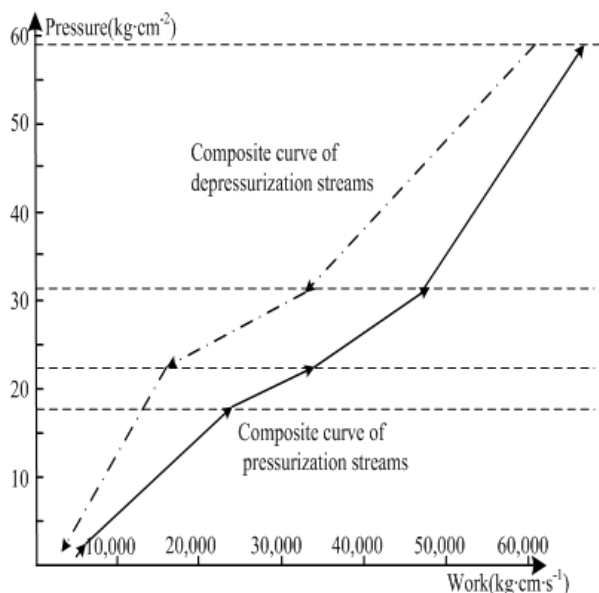
Fig. 4 Composite curves of the ammonia production process
