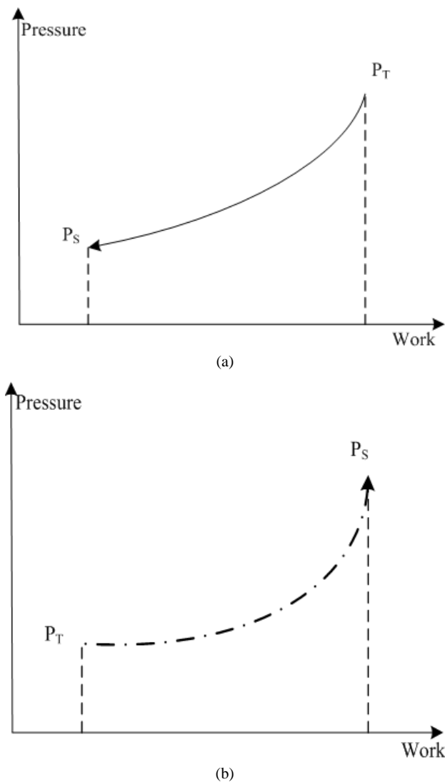
Fig. 1 A stream curve in P-W diagram
