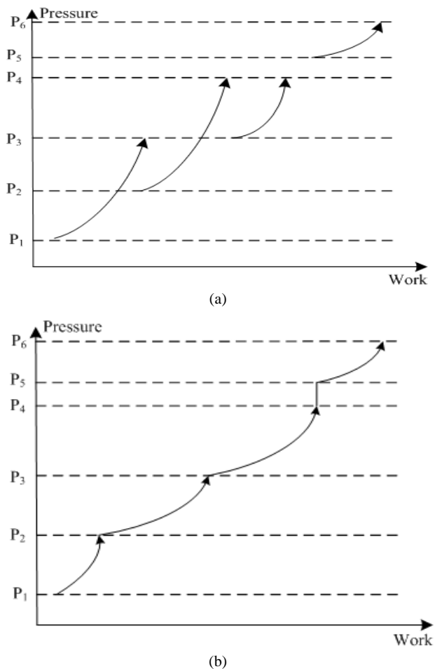
Fig. 2 The composite curve of pressurization streams
