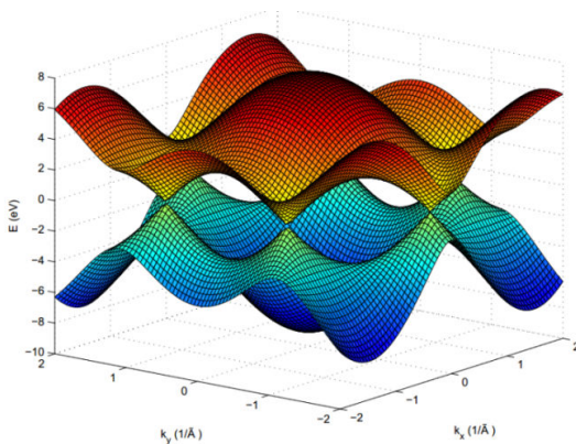
Fig. 1 The electronic dispersion in graphene
