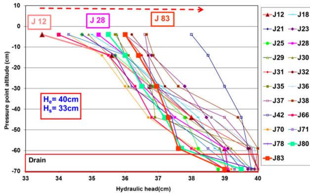
Fig. 4 (a) Evolution of the hydraulic head during the test on "material 1"
