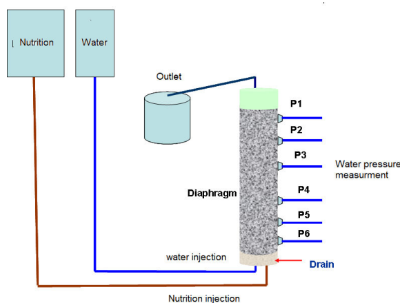
Fig. 2 Experimental device
