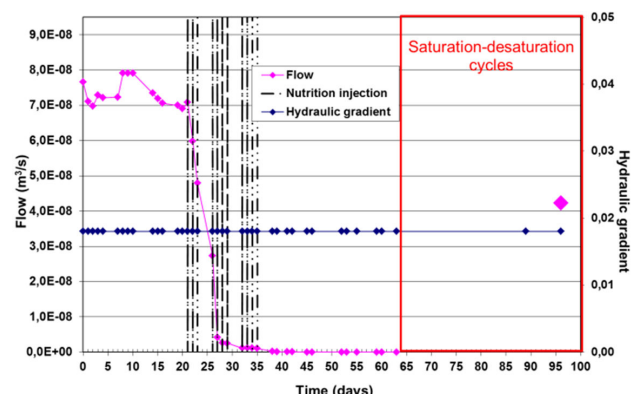
Fig. 8 (b) Evolution of the "material 2" flow during the desaturation-resaturation test
