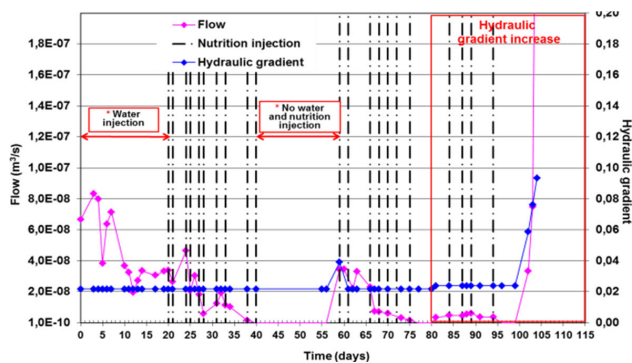
Fig. 3 (b) Evolution of the flow versus time during clogging for the "material 2"
