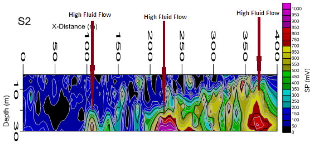
Fig. 4 SP 2D Section for Profile 2 (S2)
