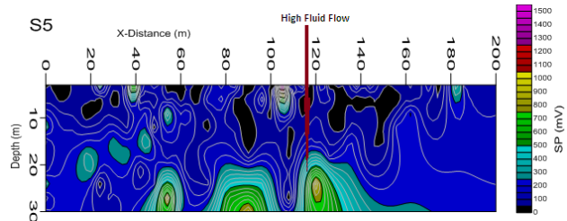
Fig. 7 SP 2D Section for Profile 5 (S5)
