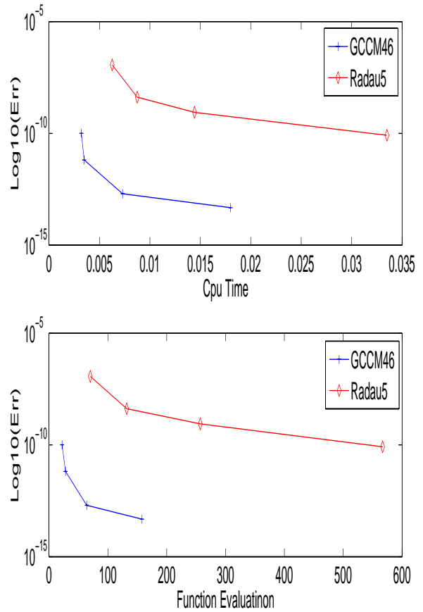
Fig. 2. Comparison of errors spent cputime (a) and versus number of function-evaluations (b)
