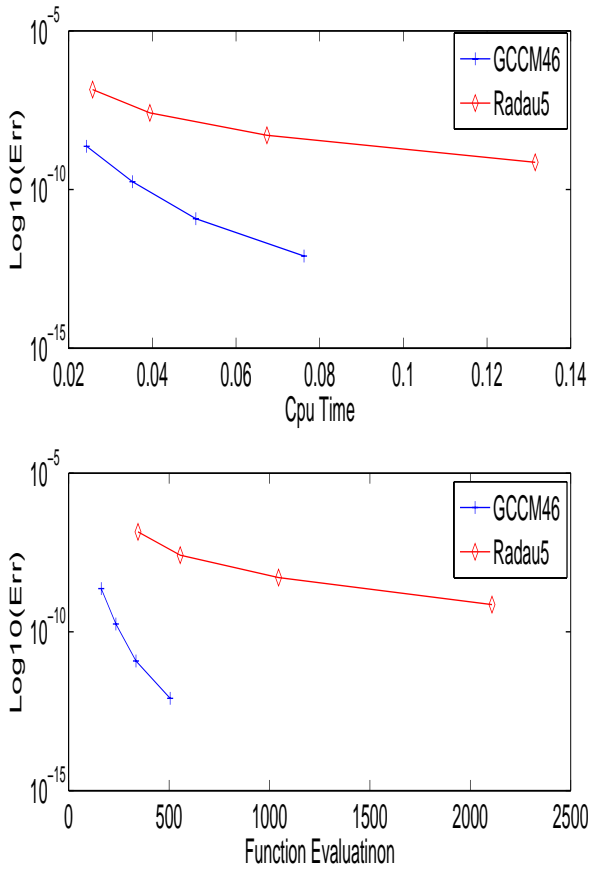
Fig. 1. Comparison of errors spent cputime (a) and versus number of function-evaluations (b)
