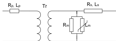
Fig. 3 Current transformer circuit diagram
