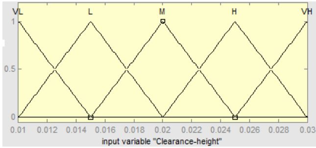
(a)clearance height
