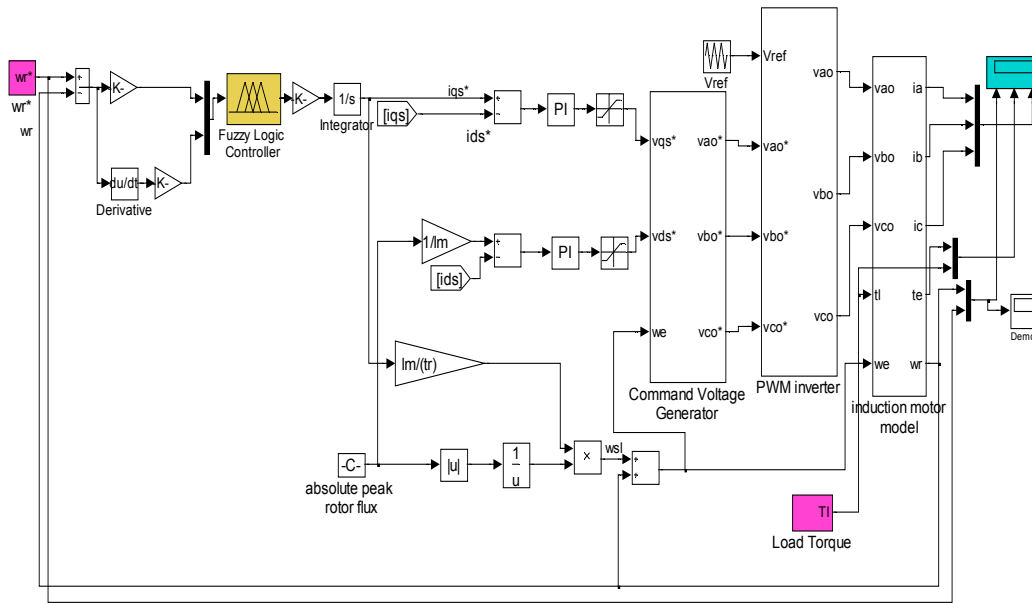
Fig. 3 Indirect vector controlled induction motor block diagram with the Fuzzy Logic Controller
