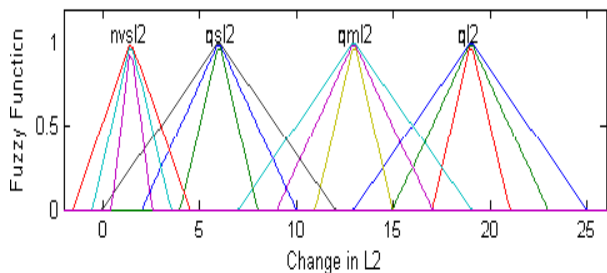
Fig. 7 Fuzzification of change in L_2
