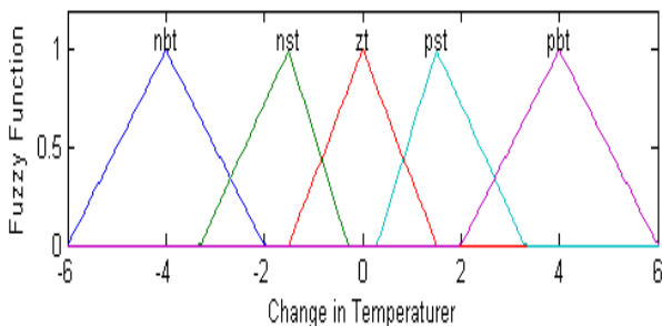
Fig. 2 Fuzzification of Change in temperature
