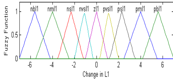
Fig. 4 Fuzzification of Change in L_1
