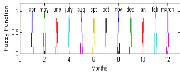
Fig. 5 Fuzzification of months
