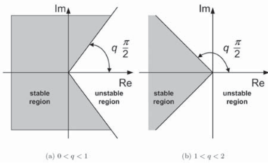
Fig. 5. Stability region of LTI fractional order systems
