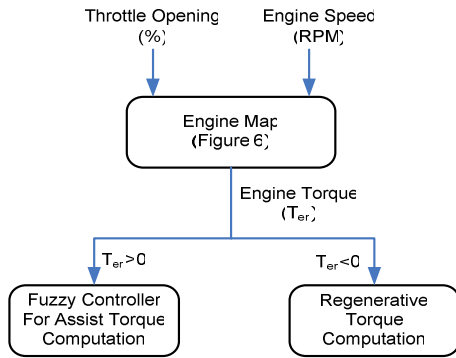
Fig. 13 Controller structure
