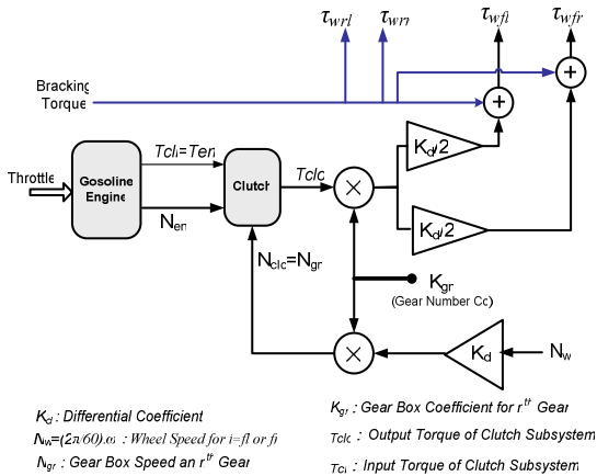
Fig. 4 Transmission subsystems modeling
