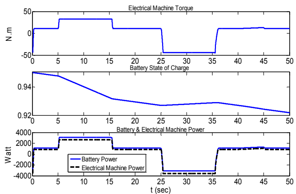
Fig. 22 Battery and electrical machine behavior
