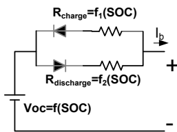
Fig. 9 The 'R_Internal' battery model
