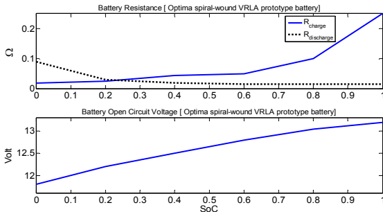
Fig. 10 Internal parameters of battery
