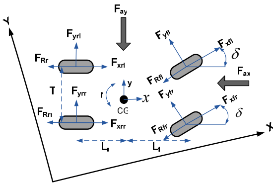
Fig. 2 Seven degrees of freedom vehicle body model
