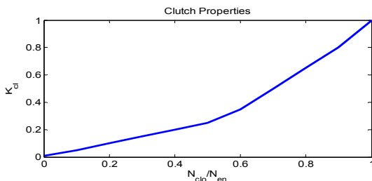
Fig. 5 Clutch power Transmission curve
