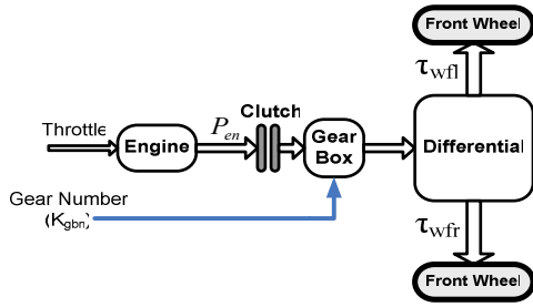
Fig. 3 Transmission subsystems structure
