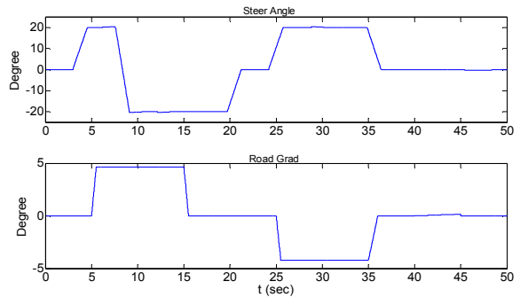
Fig. 20 Steer angle and road grad during of alpine road
