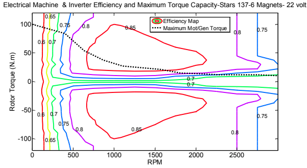
Fig. 8 Electrical machine curves
