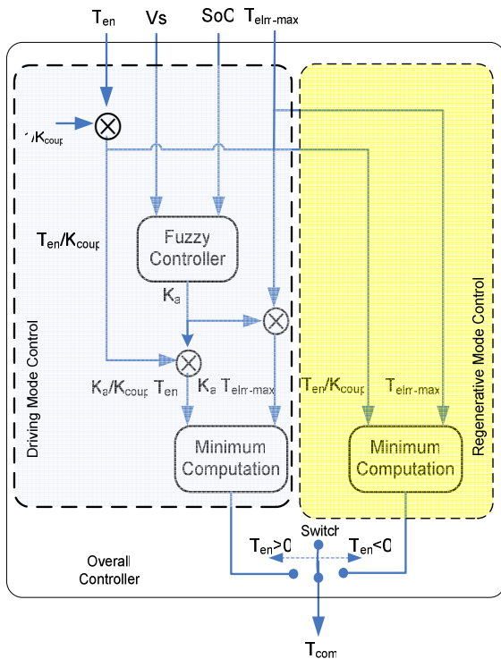
Fig. 14 Control strategy
