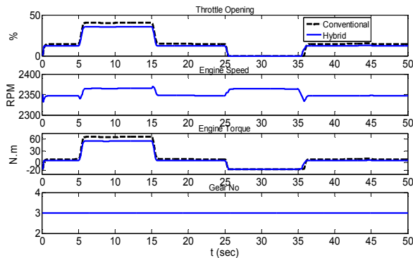
Fig. 21 Engine and gear box behavior
