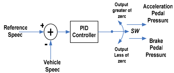
Fig. 12 Simple PID controller for pedals pressure simulation
