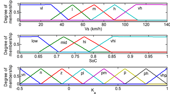
Fig. 15 Fuzzy controller memberships
