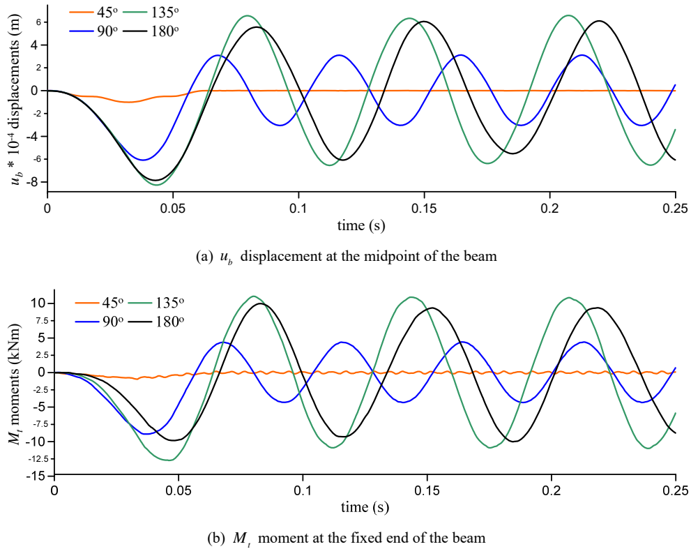
Fig. 3 Time histories of the curved beam for different values of opening angle ( \theta )
