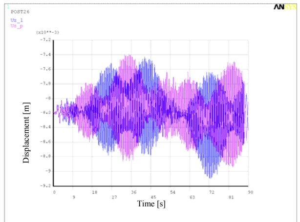
Fig. 37 Total vertical displacements, mid span U_{z_l} , U_{z_p} , Variant No. 3
