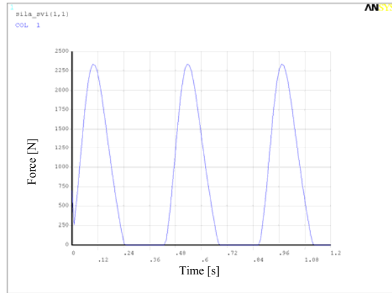
Fig. 21 Vertical force time record for running
