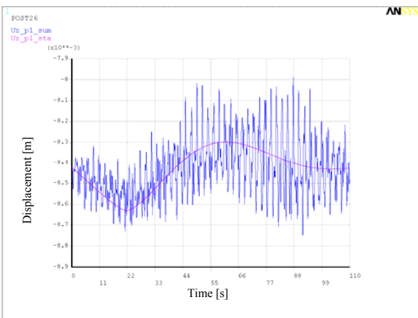
Fig. 34 Total and static vertical displacement U_z , near pylon p_1 , Variant No. 3
