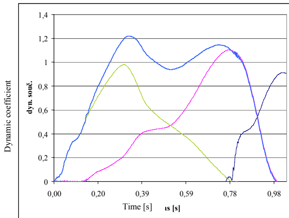
Fig. 7 Force record from gauge configuration – variant 2
