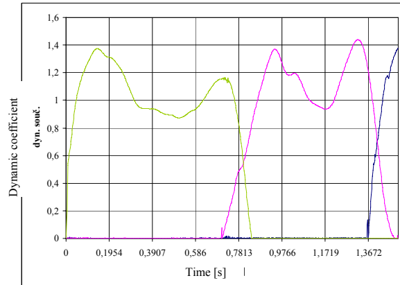
Fig. 4 Force record from gauge configuration – variant 1
