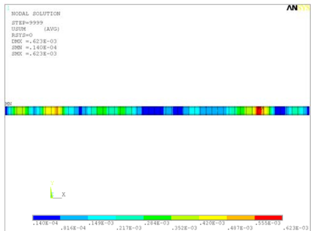
Fig. 27 Maximal envelope U_{SUM} , Variant No. 9
