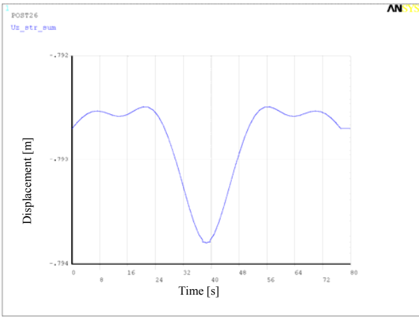
Fig. 33 Vertical displacement U_z , mid span, Variant No. 10
