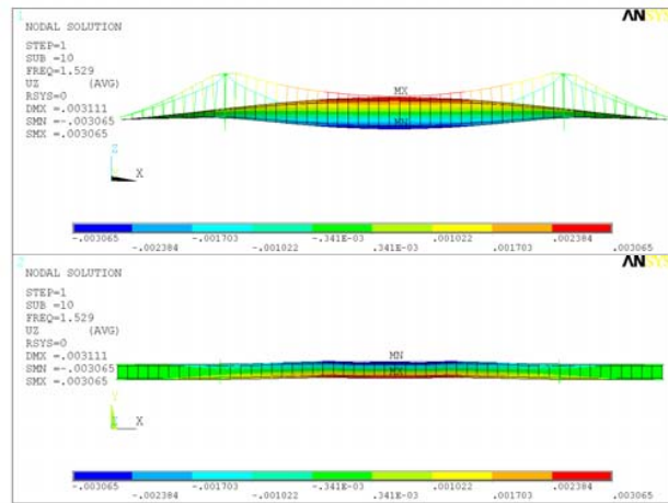
Fig. 13 Eigen shape according to f = 1.529 \text{ Hz}
