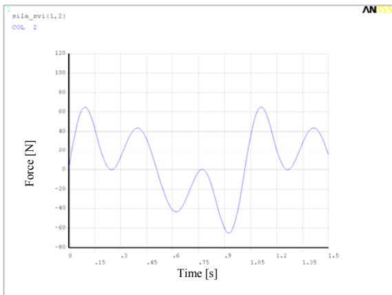
Fig. 19 Lateral force time record
