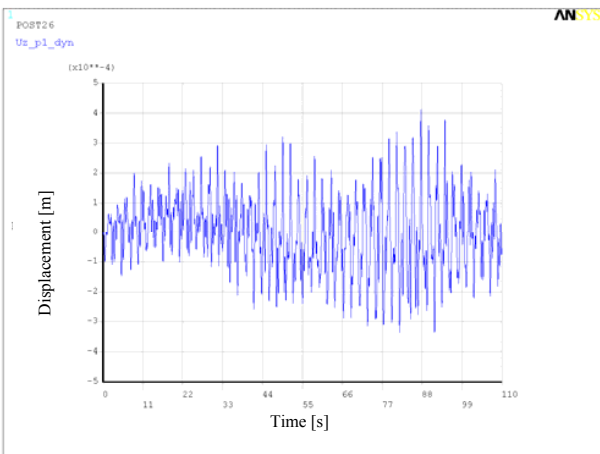
Fig. 35 Dynamic vertical displacement U_z , near pylon p_1 , Variant No. 3
