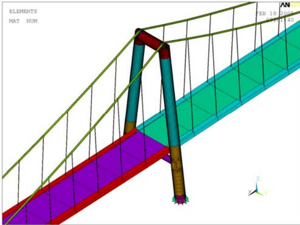
Fig. 10 Computational model – general view
