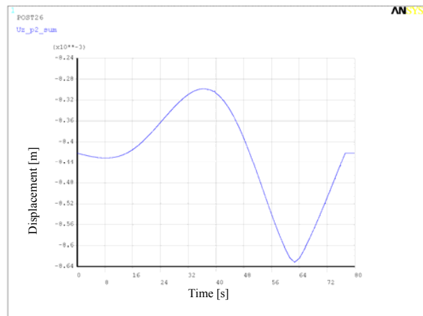
Fig. 32 Vertical displacement U_z , deck near pylon p_2 , Variant No. 10
