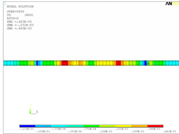
Fig. 31 Maximal envelope U_z dynamic, Variant No. 7
