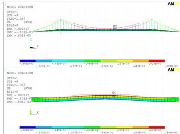
Fig. 12 Eigen shape according to f = 1.367 \text{ Hz}
