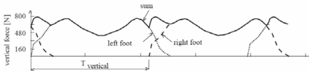
Fig. 2 General shapes for continuous vertical forces
