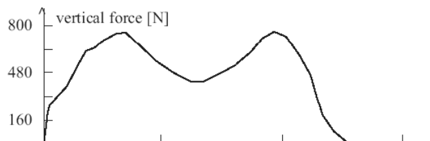
Fig. 1 Vertical force produced by one person taking one step [1].
