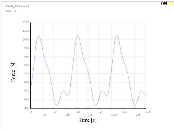
Fig. 18 Vertical force time record
