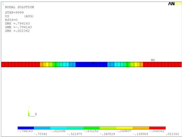
Fig. 22 Maximal envelope U_z total, Variant No. 9
