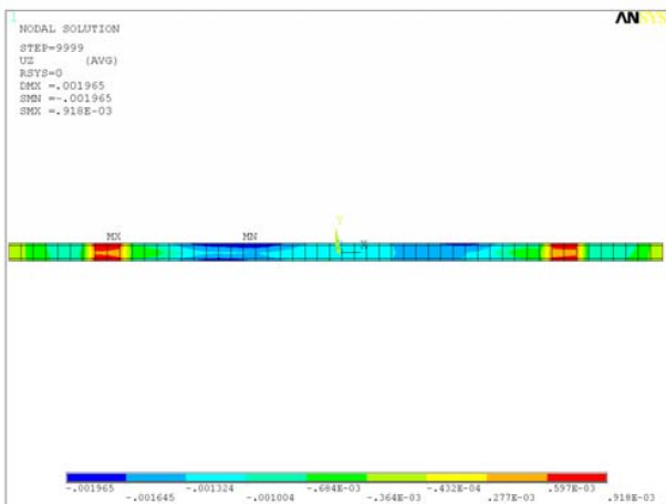
Fig. 29 Maximal envelope U_z dynamic, Variant No. 6 - second torsional
