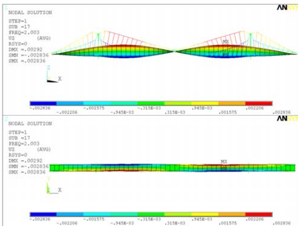
Fig. 16 Eigen shape according to f = 2.003 Hz
