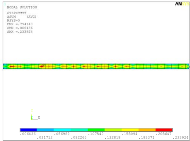
Fig. 25 Maximal envelope A_{SUM} , Variant No. 9
