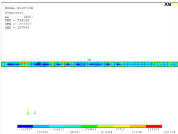
Fig. 24 Maximal envelope A_z , Variant No. 9
