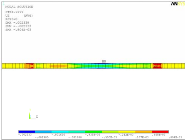
Fig. 28 Maximal envelope U_z dynamic, Variant No. 3 – torsional
