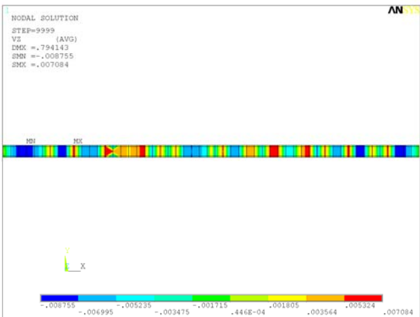
Fig. 23 Maximal envelope V_z , Variant No. 9
