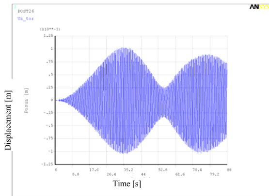
Fig. 39 Displacements difference for U_{z_l} and U_{z_p} , Variant No. 6
