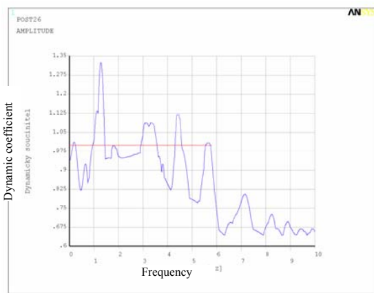
Fig. 8 Force-frequency record
