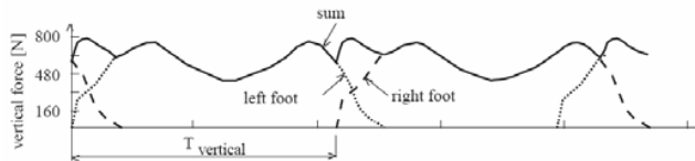
Fig. 2 General shapes for continuous vertical forces
