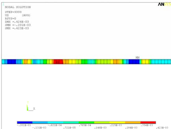
Fig. 30 Maximal envelope U_z dynamic, Variant No. 2
