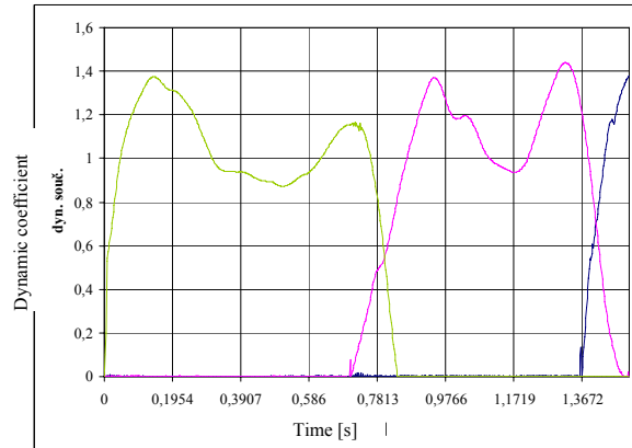
Fig. 4 Force record from gauge configuration – variant 1
