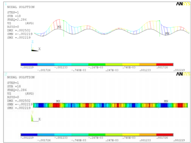
Fig. 17 Eigen shape according to f = 2.286 Hz
