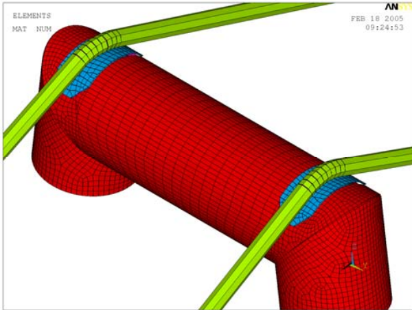
Fig. 11 Computational model – detail view
