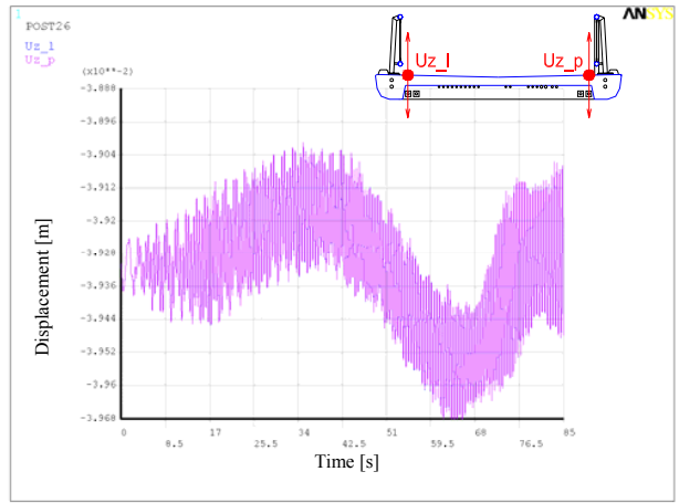
Fig. 36 Total vertical displacements, mid span U_{z_l} , U_{z_p} , Variant No. 2
