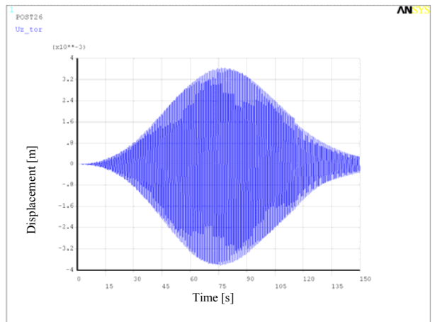
Fig. 38 Displacements difference for U_{z_l} and U_{z_p} , Variant No. 3
