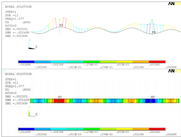
Fig. 14 Eigen shape according to f = 1.677 Hz
