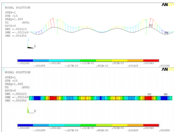
Fig. 15 Eigen shape according to f = 1.965 Hz
