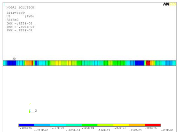
Fig. 26 Maximal envelope U_z dynamic, Variant No. 9
