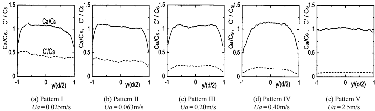
Fig. 8 Distributions of fiber concentration on y-axis ( C_s = 0.6\% )
