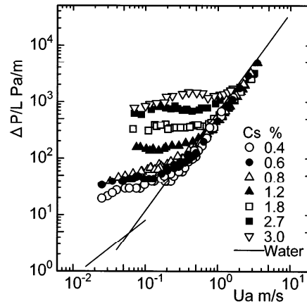
Fig. 5 Pressure losses for several concentrations of pulp-suspension
