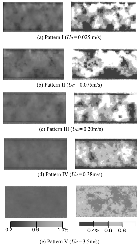
Fig. 3 Influence of average velocity on the distribution of fiber concentration ( C_S = 0.6\% ). Left and right figures show the distributions and four-level ones of fiber concentration, respectively.
