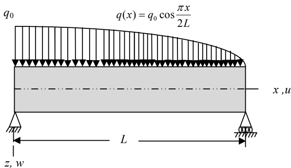
Fig. 2 Simply supported beam with cosine load
