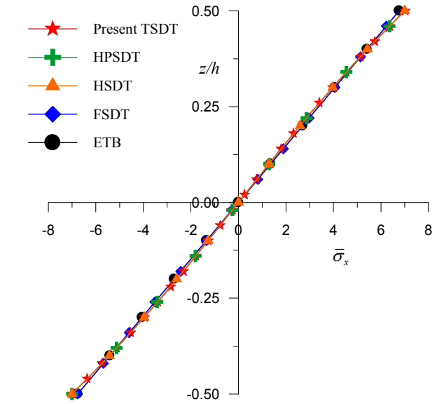
Fig. 6 Variation of axial stress ( \bar{\sigma}_x ) through the thickness of simply supported beam at ( x = 0.25L, z ) when subjected to cosine load for aspect ratio 4 (Example 1)
