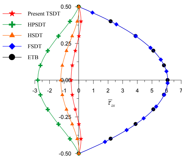
Fig. 11 Variation of transverse shear stress ( \bar{\tau}_{zx} ) through the thickness of simply supported beam at (x = 0, z) when subjected to cosine load and obtain using equilibrium equation for aspect ratio 10 (Example 1)
