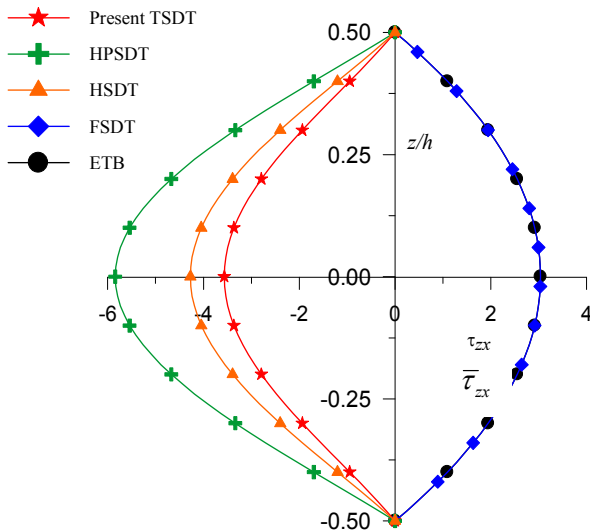
Fig. 21 Variation of transverse shear stress ( \bar{\tau}_{zx} ) through the thickness of simply supported beam at (x=0, z) when subjected to cosine load and obtain using equilibrium equation for aspect ratio 10 (Example 2)
