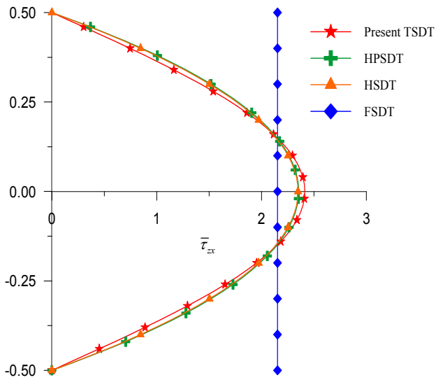
Fig. 8 Variation of transverse shear stress ( \bar{\tau}_{zx} ) through the thickness of simply supported beam at (x = 0, z) when subjected to cosine load and obtain using constitutive relation for aspect ratio 4 (Example 1)
