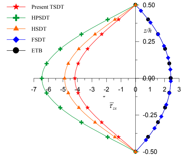
Fig. 10 Variation of transverse shear stress ( \bar{\tau}_{zx} ) through the thickness of simply supported beam at (x = 0, z) when subjected to cosine load and obtain using equilibrium equation for aspect ratio 4 (Example 1)
