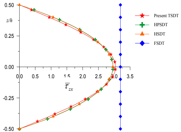
Fig. 19 Variation of transverse shear stress ( \bar{\tau}_{zx} ) through the thickness of simply supported beam at ( x = 0, z ) when subjected to cosine load and obtain using constitutive relation for aspect ratio 10 (Example 2)
