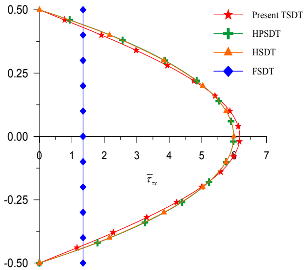
Fig. 9 Variation of transverse shear stress ( \bar{\tau}_{zx} ) through the thickness of simply supported beam at (x = 0, z) when subjected to cosine load and obtain using constitutive relation for aspect ratio 10 (Example 1)
