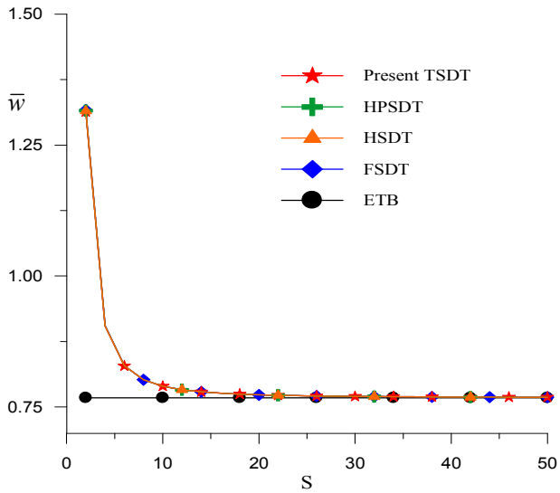
Fig. 12 Variation of maximum transverse displacement ( \bar{w} ) of simply supported beam at ( x = 0.25L, z = 0 ) when subjected to cosine load with aspect ratio S (Example 1)
