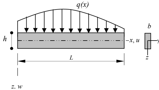
Fig. 1 Beam under bending in x - z plane
