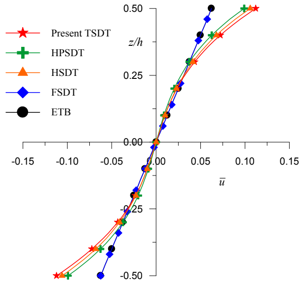
Fig. 14 Variation of axial displacement ( \bar{u} ) through the thickness of simply supported beam at ( x = 0.25L, z ) when subjected to cosine load for aspect ratio 4 (Example 2)
