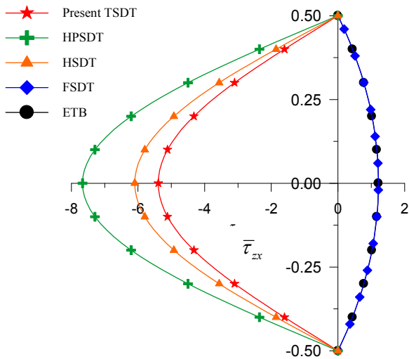
Fig. 20 Variation of transverse shear stress ( \bar{\tau}_{zx} ) through the thickness of simply supported beam at (x=0, z) when subjected to cosine load and obtain using equilibrium equation for aspect ratio 4 (Example 2)
