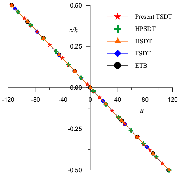
Fig. 5 Variation of axial displacement ( \bar{u} ) through the thickness of simply supported beam at ( x = 0.25L, z ) when subjected to cosine load for aspect ratio 10 (Example 1)
