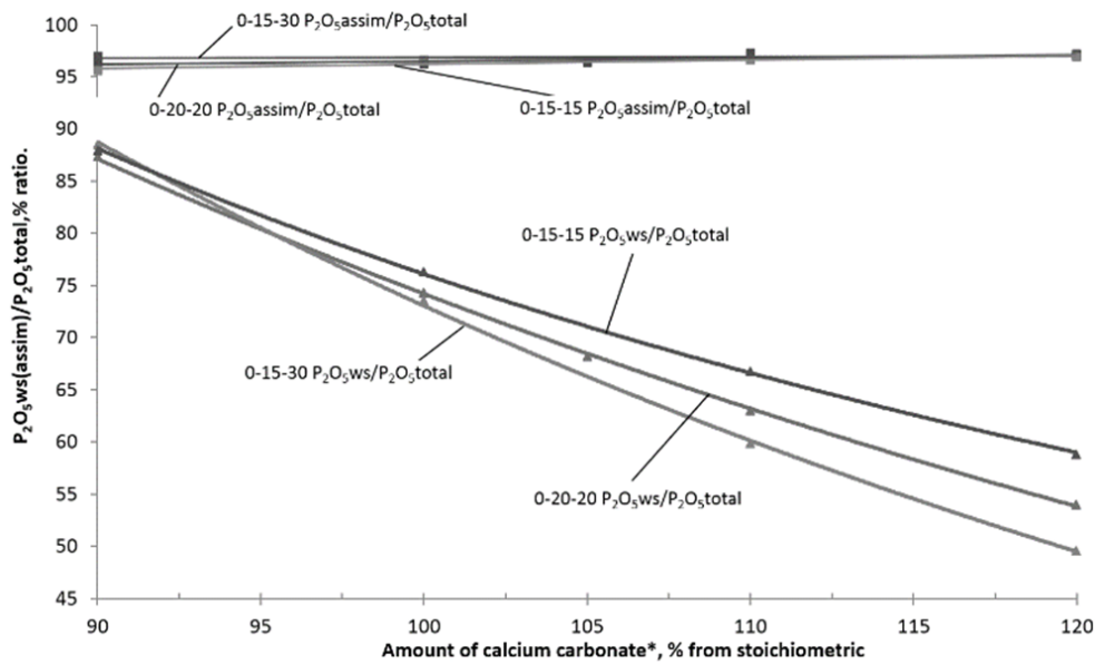
Fig. 4 Dependence of ratios of P_2O_{5\text{ws}}/P_2O_{5\text{total}} & P_2O_{5\text{assim}}/P_2O_{5\text{total}} in PKS-fertilizers of various grades on amount of calcium carbonate supplied for acid neutralization
