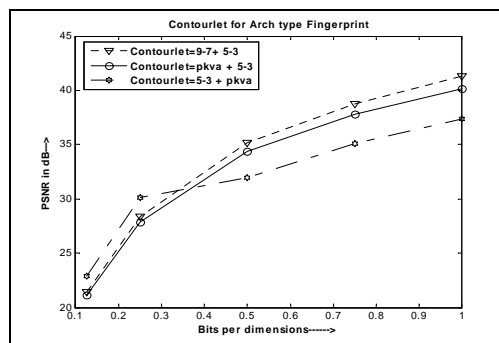
Fig. 10 Comparison of bit rate Vs PSNR between different pyramid and directional filters for Arch type Fingerprint
