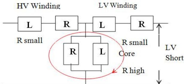
Fig. 2 Short circuit model
