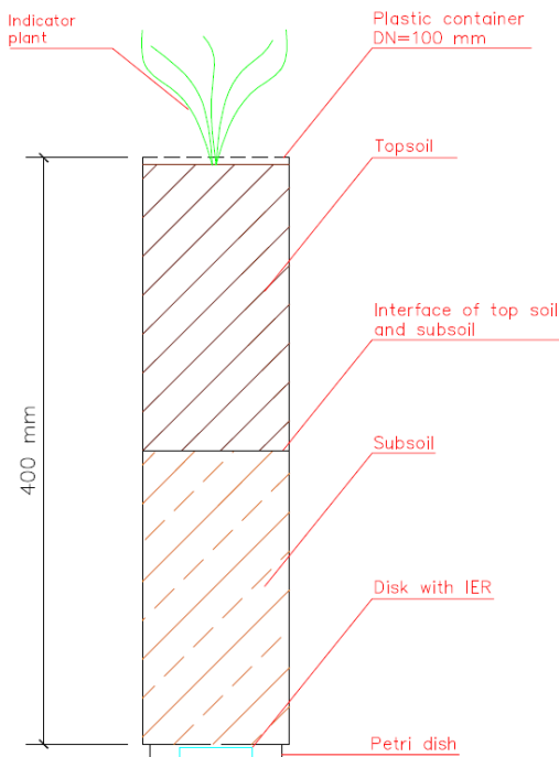
Fig. 1 Experimental container
