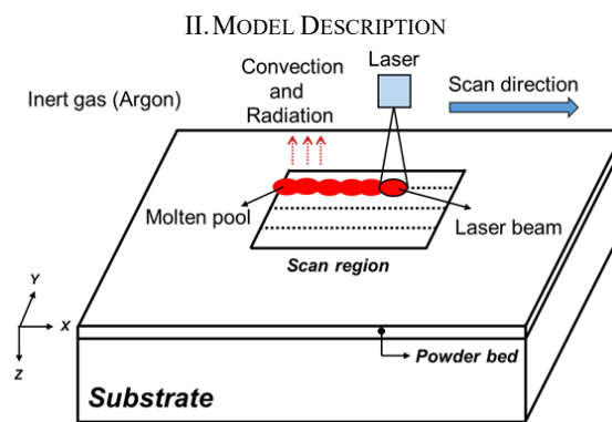
Fig. 1 Schematic of the heat transfer mechanism for laser heating of metal powders
