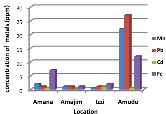
Fig. 2 Comparison of the mean concentration of the metals based on location
