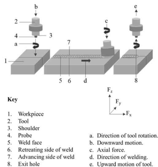
Fig. 1 Operating principle and components of conventional FSW
