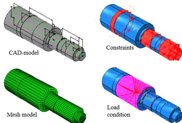
Fig. 5 Shaft modeling
