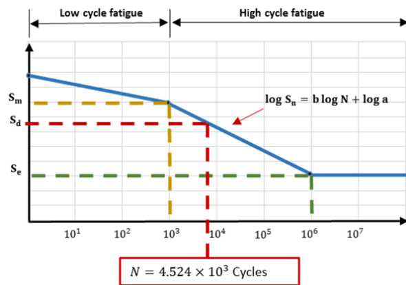
Fig. 4 Calculated stress-cycle (s-n) diagram
