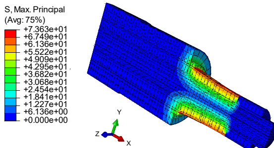
Fig. 7 Shaft shear stresses
