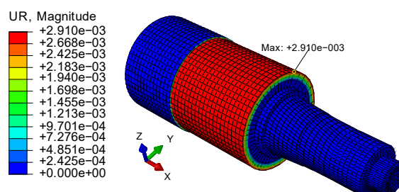
Fig. 9 Shaft torsional deflection
