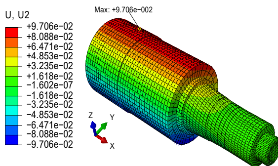
Fig. 8 Shaft bending deflection
