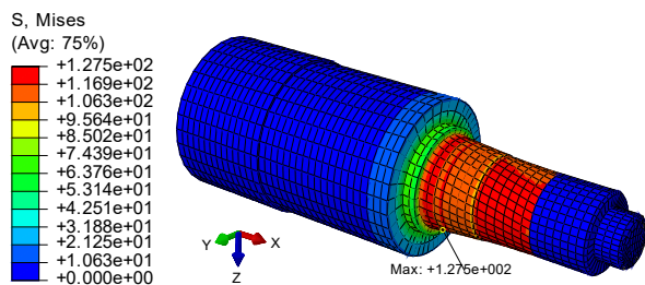
Fig. 6 Shaft equivalent stresses (von Mises)
