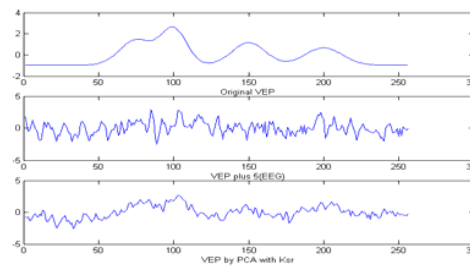
Fig. 5 Artificial VEP signals with PCs selected using KSR (EEG factor of 5)
