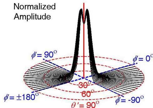
Fig. 4. Calculated radiation pattern of TSFF5200 LED.
