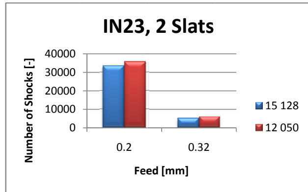
Fig. 4 Dependence of number of shocks on feed at 2 slats
