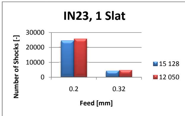
Fig. 5 Dependence of number of shocks on feed at 1 slat
