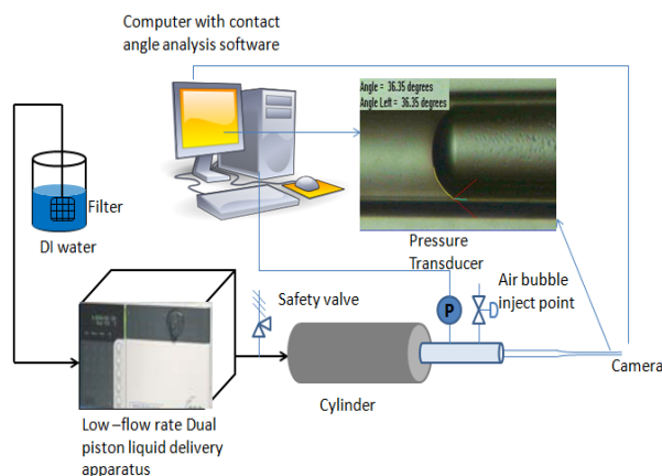
Fig. 1 Mutiphase flow transport experimental setup
