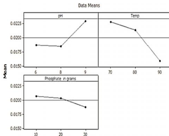
Fig. 10 Main effects plot for impact energy
