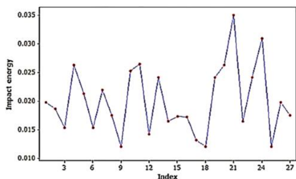
Fig. 9 Time series plot for impact energy
