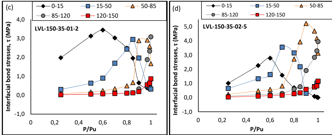
Fig. 4 Relationship between bond stress and bond thickness
