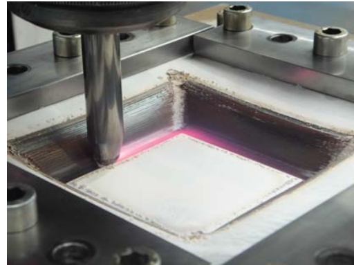
Fig. 3 IASPIF process during pyramid profile forming and induction heating
