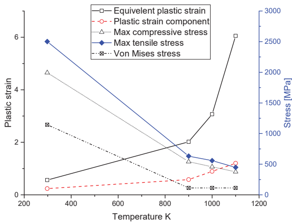
Fig. 9 The influence of heating temperature on the stress strain components for pyramid of DP980 steel
