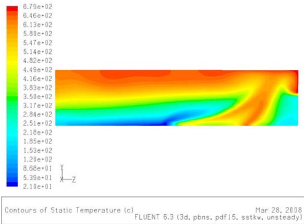
Contours of Static Temperature (c) Mar 28, 2008 FLUENT 6.3 (3d, pbns, pdf15, sstk, unsteady) Fig. 7 CFD predicted temperature distribution at time t=13 s of combustion on the centerline plane of fuel source (Q=2 kW, V_c=1.41 m/s, V_{inlet}=1 m/s)
