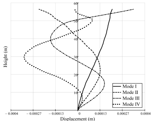
Fig. 13 Displacement evaluation on Model 1
