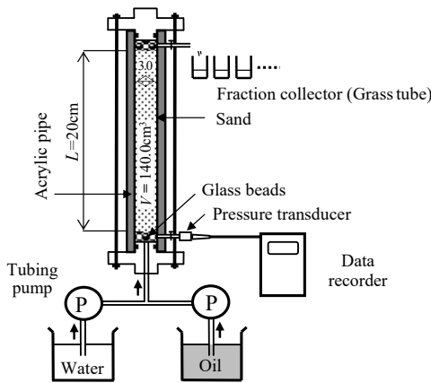
Fig. 2 Experimental apparatus
