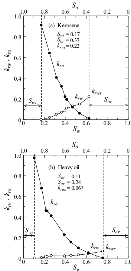
Fig. 5 Relative permeability curves for water displacement by oils
