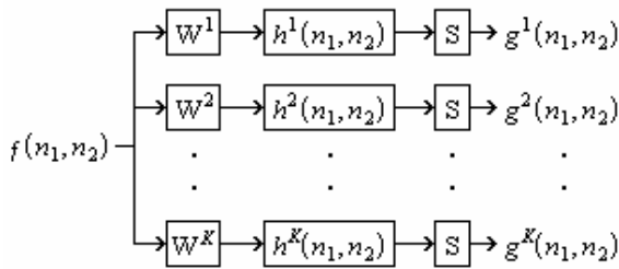
Fig. 1 Observation model
