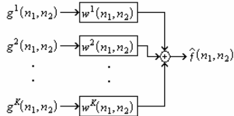
Fig. 2 Reconstruction stage
