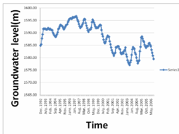
Fig. 2 The groundwater hydrograph(m) of Arsanjan plain
