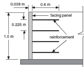
Fig. 1 The schematic view of GRSRW in shaking table experiment
