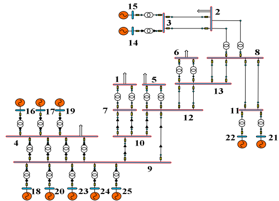
Fig. 1 Single line diagrams for the 25-bus equivalent practical power system
