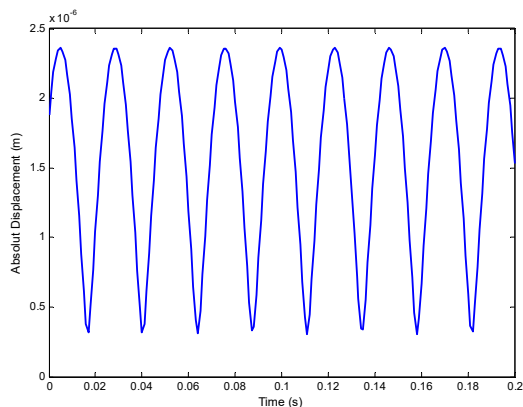
Fig. 8 Absolute radial displacement of spindle-bearing (optimized)
