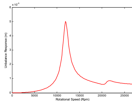
Fig. 3 Unbalance response of spindle system
