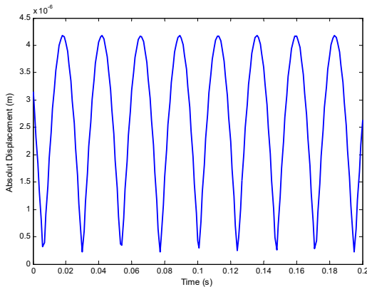
Fig. 5 Absolute radial displacement of spindle (before)
