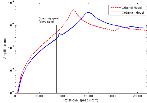
Fig. 6 Comparison of unbalance response
