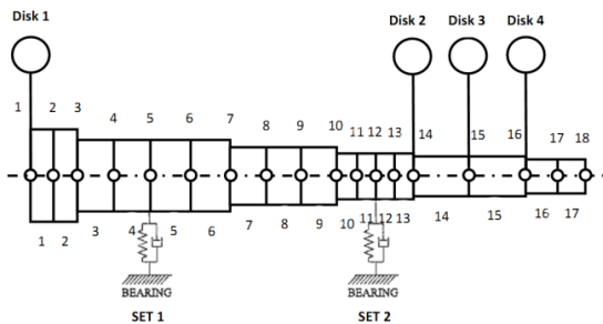
Fig. 2 Finite element model (FEM) of spindle system
