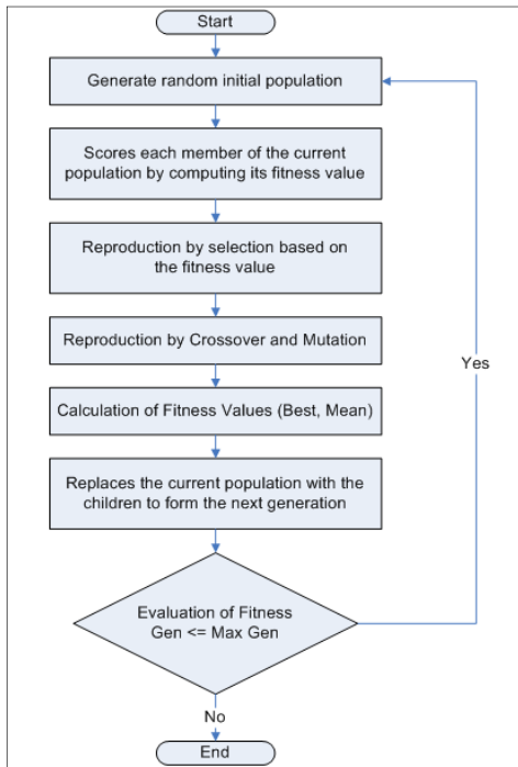
Fig. 1 Flowchart of genetic algorithm (GA)
